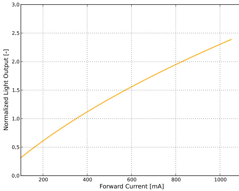
Figure 4b: Typical normalized light output vs. forward current for LUXEON C PC Amber at T_j=85^\circ\text{C} .
