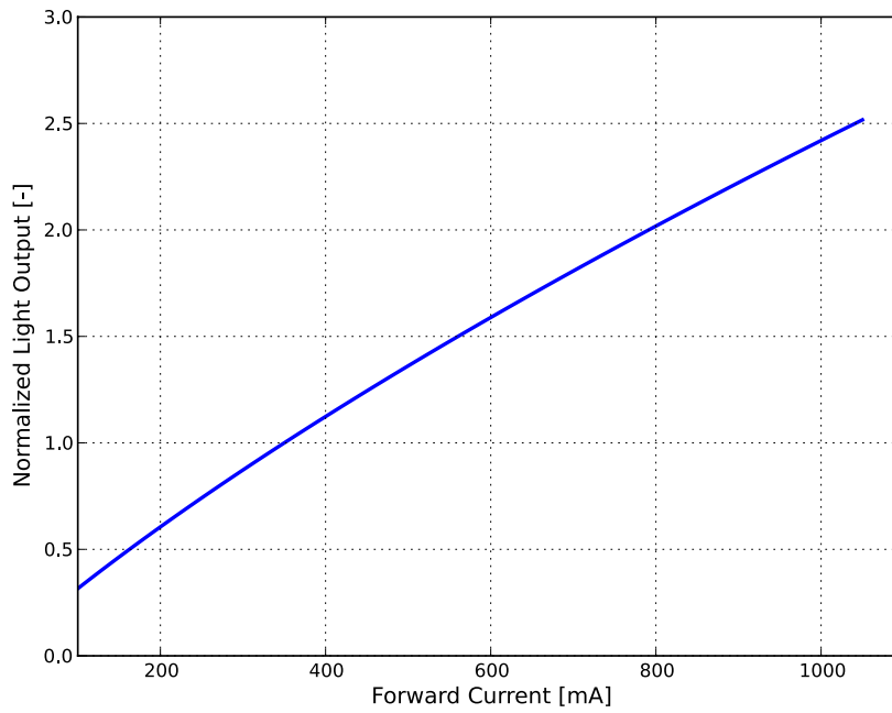
Figure 4d: Typical normalized light output vs. forward current for LUXEON C Royal Blue at T_j=85^\circ\text{C} .
