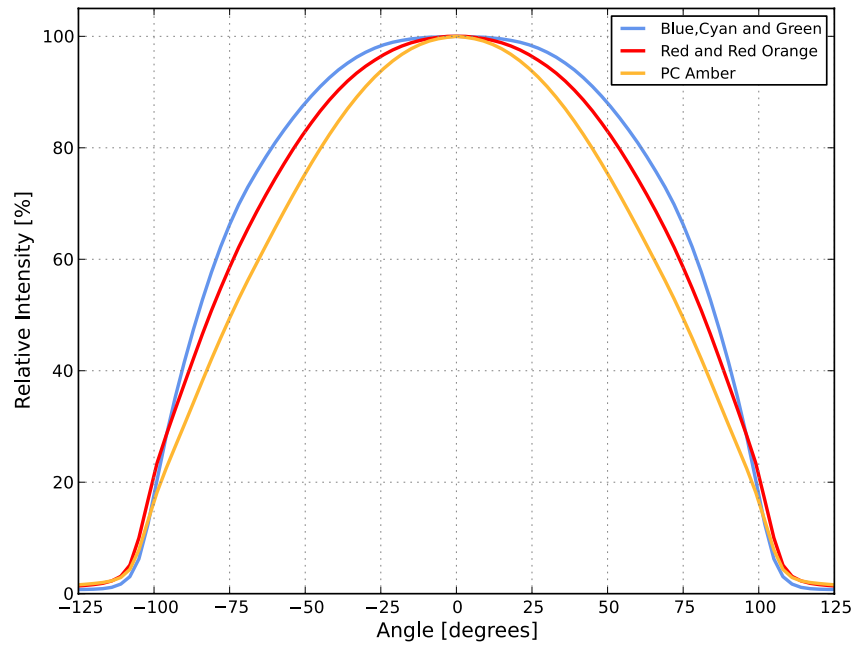
Figure 6a: Typical radiation pattern for LUXEON C Red, Red-Orange, PC Amber, Cyan, Green and Blue at 350mA, T_j=85^\circ\text{C} .
