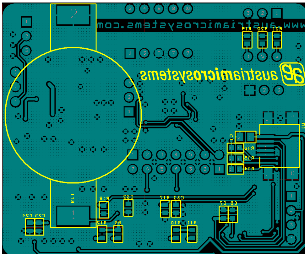
Figure 5: Bottom Layer
